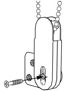
Inside Mount
